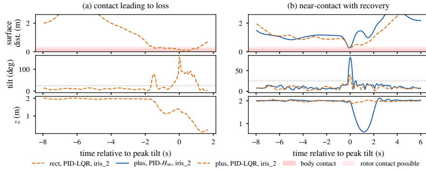
FIGURE 9. Upsets aligned at peak tilt: surface distance to the nearest static cylinder (dark: body contact; light: rotor contact possible), tilt (dotted: 25^\circ level-out) and altitude. (a) PID-LQR, rect, agent 2: contact and loss. (b) plus , agent 2, both controllers: graze and recovery.
